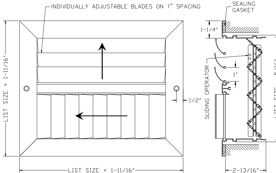
Standard blade option shown. See Curved Blade Options page.
