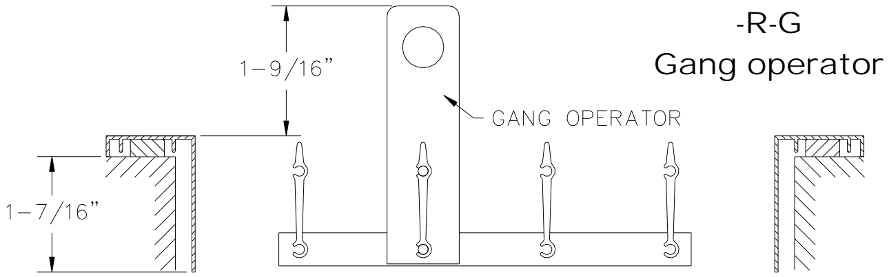
Gang operator can extend out up to 1-9/16". Do not specify this blade option for a location where it may cause a safety concern. Extra operator installed every 26". Only available with -R recessed blade option.
